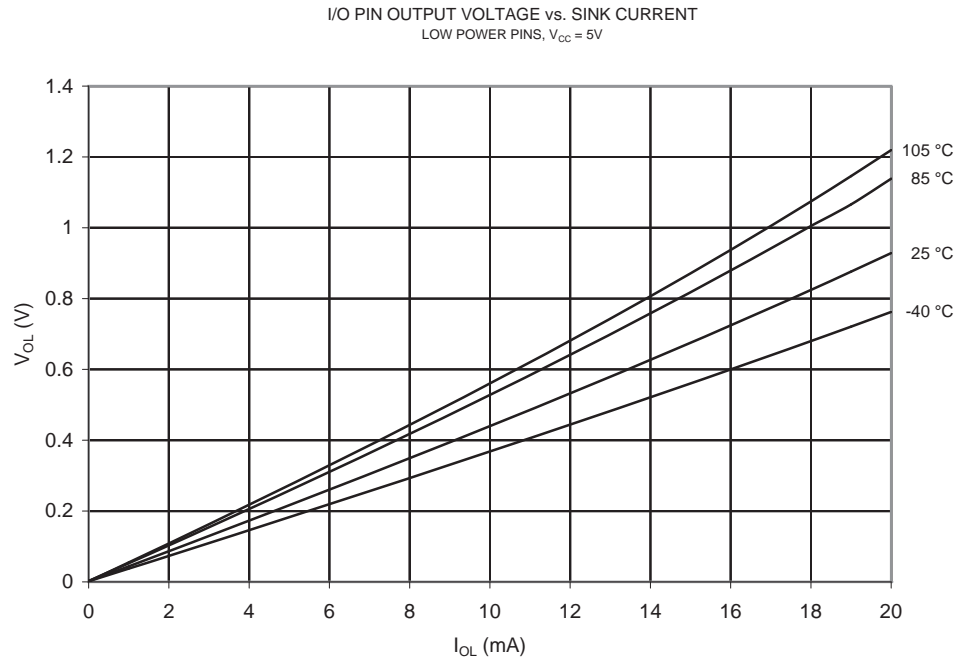
Figure 2-26. V_{OL} : I/O Pin Output Voltage vs. Sink Current (Low Power Pins, V_{CC} = 5V )
