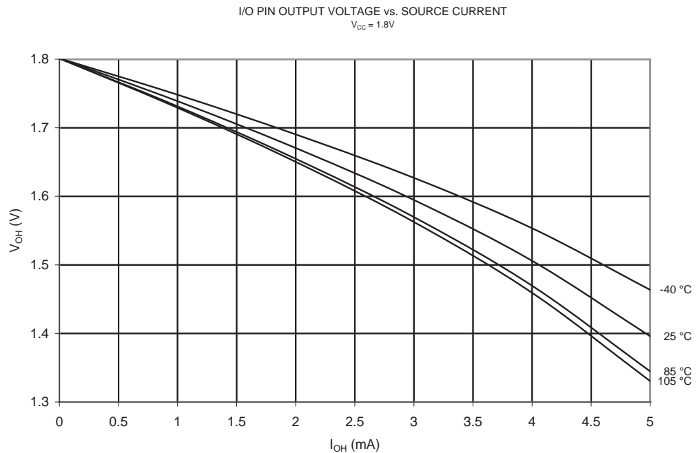
Figure 2-27. V_{OH} : I/O Pin Output Voltage vs. Source Current ( V_{CC} = 1.8V )
