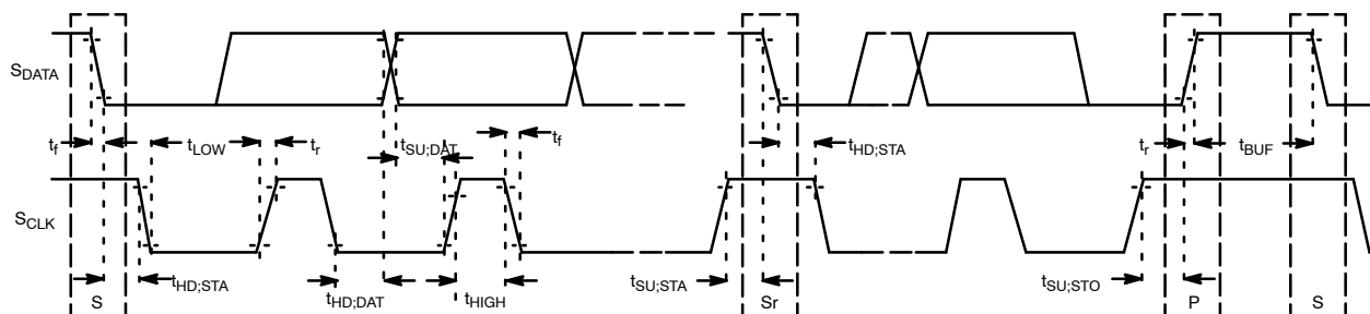
Figure 26. Slave Two Wire Serial Bus Timing Parameters (CCIS)
