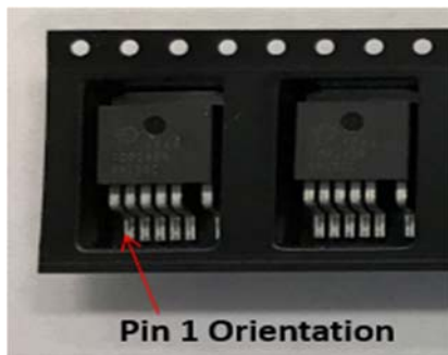
Current Pin 1 Orientation
