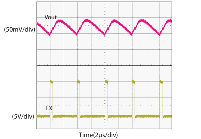
Forced Continuous Mode - No Load V IN = 12 V, V OUT = 1.2 V, I OUT = 0 A, V DD = EN/PSV = ENL = 5 V
