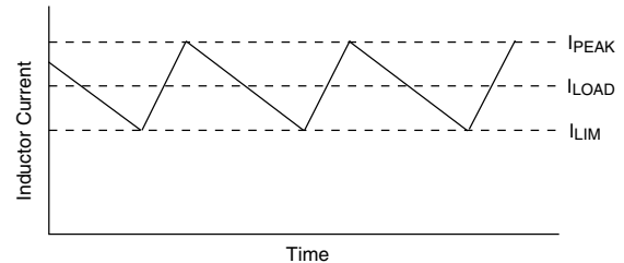
Fig. 8 - Valley Current Limit
