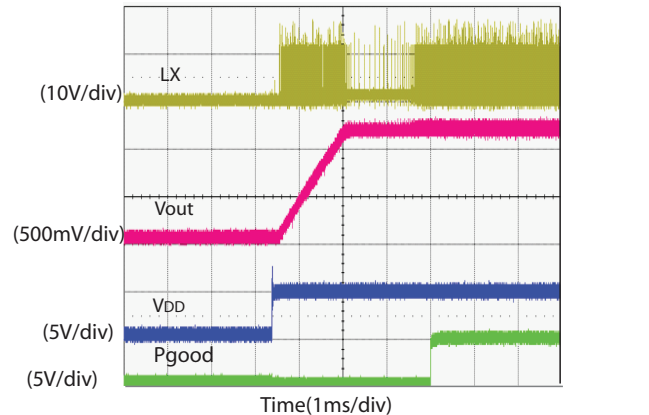
Enable Start-Up - Power Good True V IN = 12 V, V OUT = 1.2 V, I OUT = 1 A, V DD = EN/PSV = 5 V
