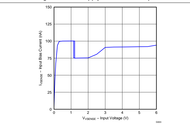
Figure 4. VSENSE Input Bias Current vs Input Voltage
