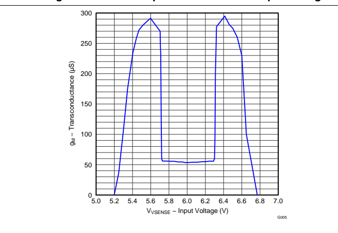
Figure 6. Error Amplifier Transconductance vs VSENSE
