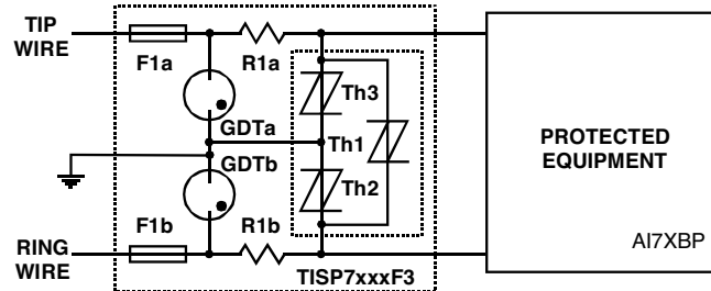
Figure 20. Protection Module
