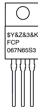
TO-220 CASE 340AT
