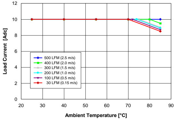
Fig. 5.0V.1: Available load current vs. ambient temperature and airflow rates for V_{out} = 5.0\text{ V} converter mounted vertically with V_{in} = 12\text{ V} , and maximum MOSFET temperature \leq 110\text{ }^\circ\text{C} .
