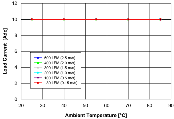
Fig. 2.0V.1: Available load current vs. ambient temperature and airflow rates for V_{out} = 2.0\text{ V} converter mounted vertically with V_{in} = 12\text{ V} , and maximum MOSFET temperature \leq 110\text{ }^{\circ}\text{C} .
