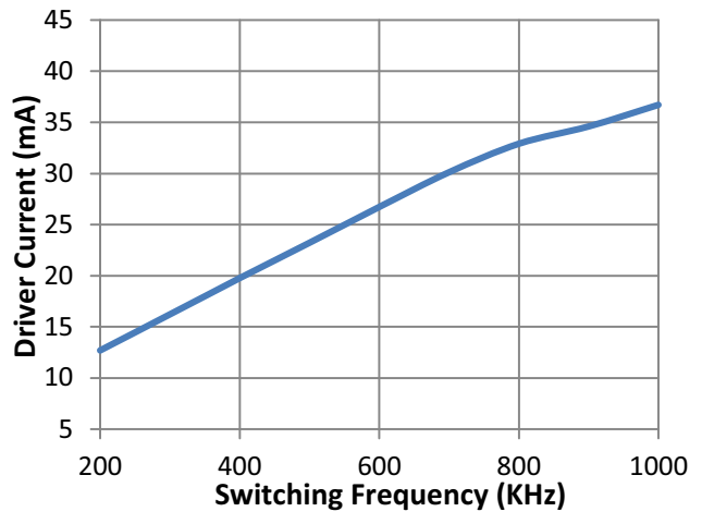
Figure 9. Driver Supply Current vs. Switching Frequency
