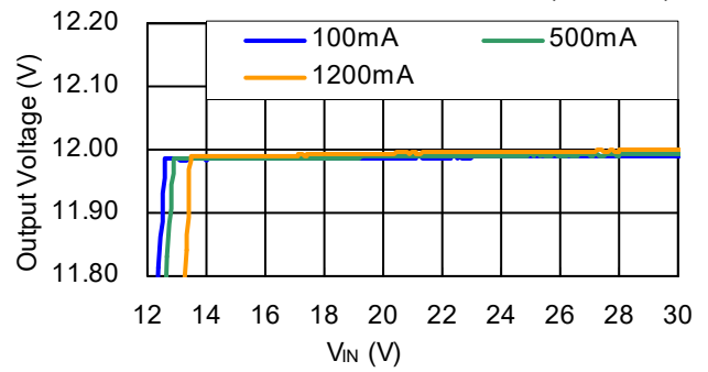
R1245x00xC/R1245x00xD V_{OUT}=12V
