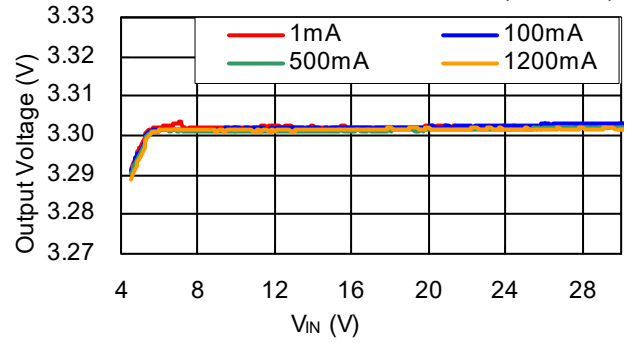
R1245x00xC/R1245x00xD V_{OUT}=3.3V
