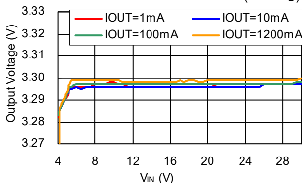
R1245x00xA/R1245x00xB
