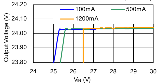
R1245x00xC/R1245x00xD V_{OUT}=24V
