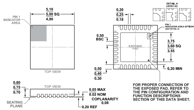
Figure 70. 32-Lead Lead Frame Chip Scale Package [LFCSP] 5 mm × 5 mm Body and 0.75 mm Package Height (CP-32-12) Dimensions shown in millimeters
