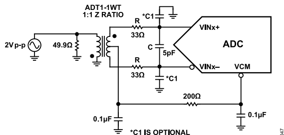
Figure 56. Differential Transformer-Coupled Configuration for Baseband Applications
