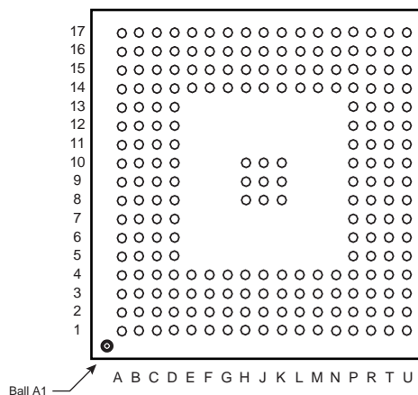
Figure 3-1. 217-ball LFBGA Package Outline (Top View)
